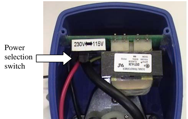
Figure 1. Input Voltage Switch
